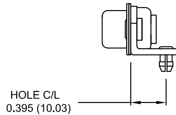
50 POSITION CONNECTOR BRACKET
