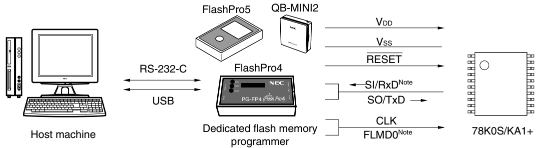
Figure 18-2. Environment for Writing Program to Flash Memory (FlashPro4/FlashPro5/QB-MINI2)
