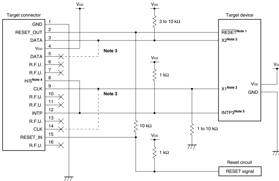
Figure 19-1. Recommended Circuit Connection
