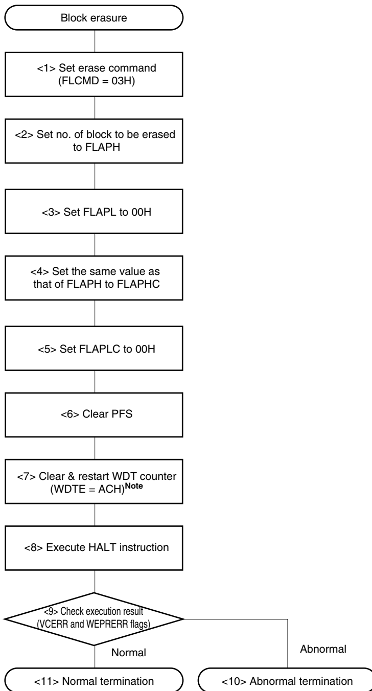
Figure 18-20. Example of Block Erase Operation in Self Programming Mode
