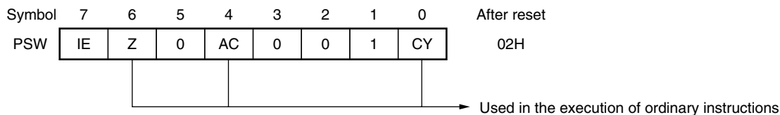
Figure 12-6. Program Status Word (PSW) Configuration
