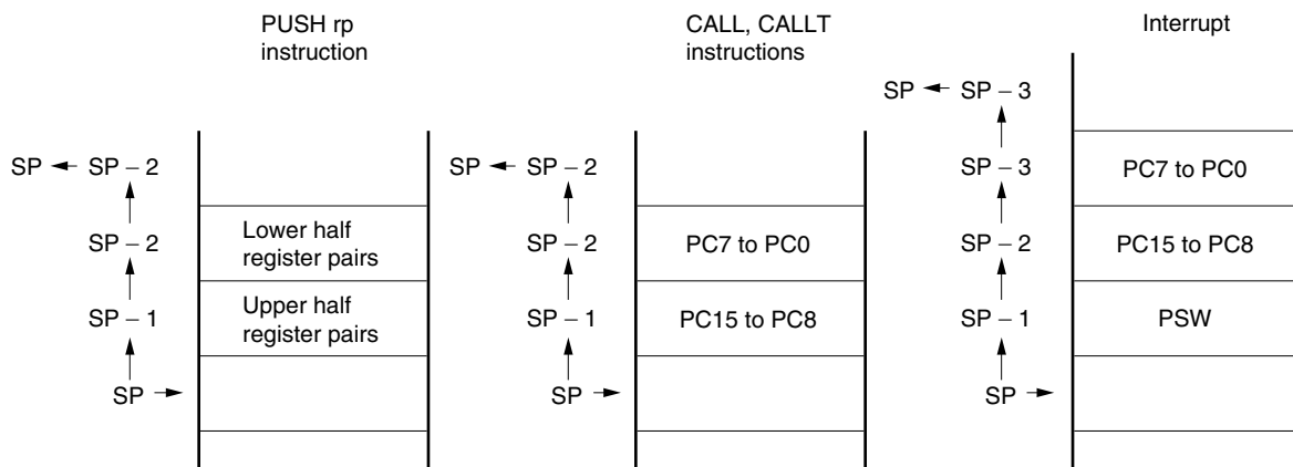
Figure 3-8. Data to Be Saved to Stack Memory
