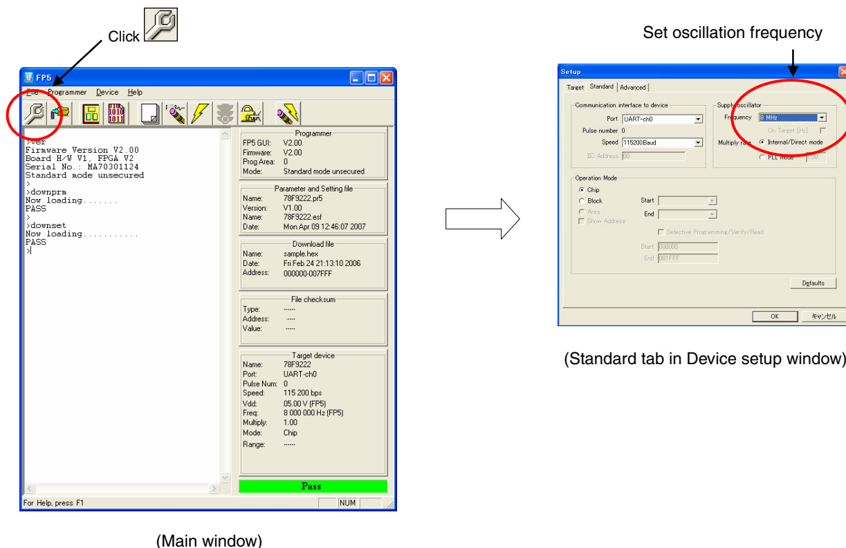
Figure 18-5. PG-FP5 GUI Software Setting Example
