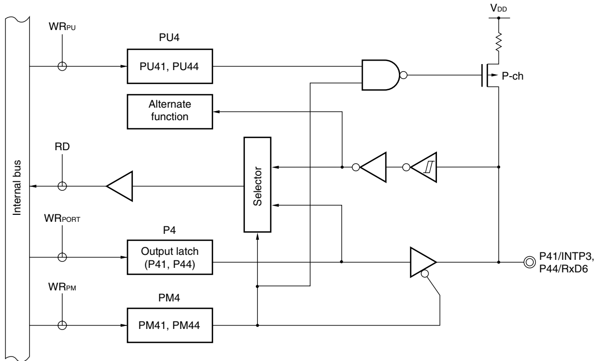
Figure 4-7. Block Diagram of P41 and P44
