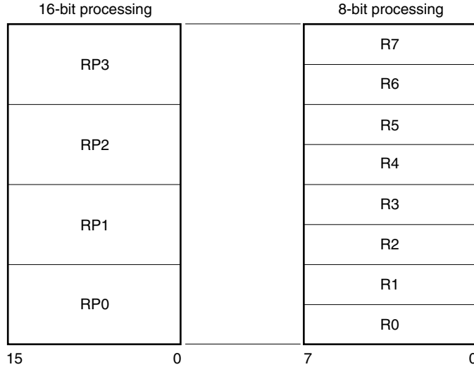
Figure 3-10. General-Purpose Register Configuration (2/2) (b) Absolute names
