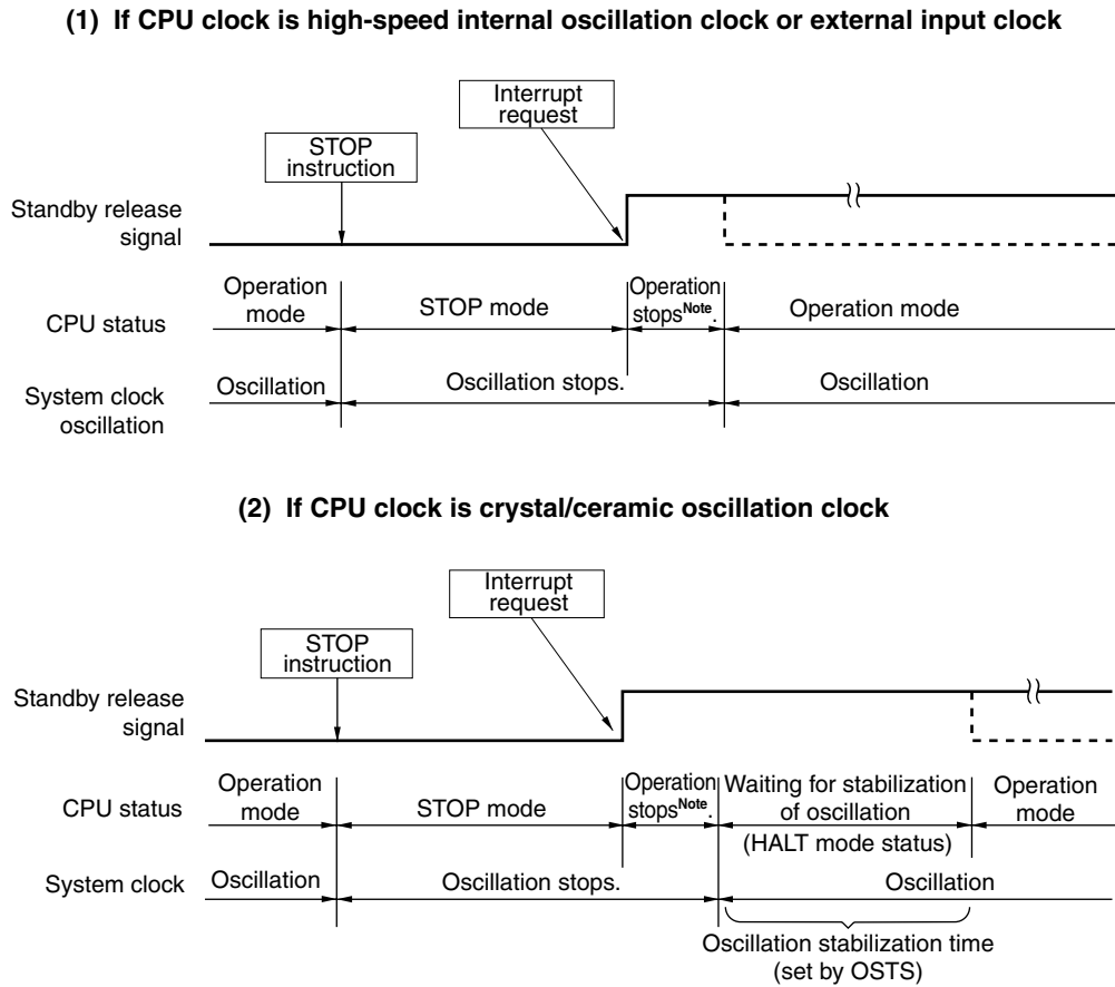
Figure 13-5. STOP Mode Release by Interrupt Request Generation
