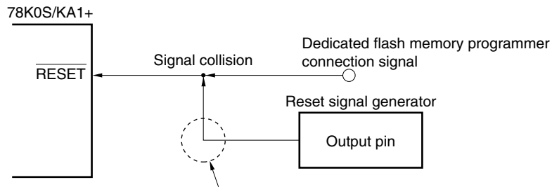
Figure 18-6. Signal Collision ( \overline{\text{RESET}} Pin)
