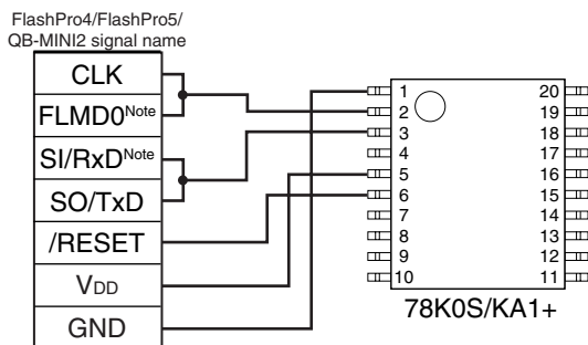
Figure 18-3. Wiring diagram with FlashPro4/FlashPro5/QB-MINI2
