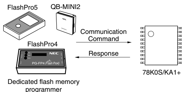
Figure 18-7. Communication Commands
