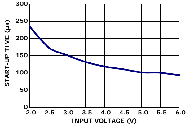
FIGURE 18. START-UP TIME vs SUPPLY VOLTAGE
