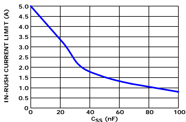
FIGURE 39. IN-RUSH CURRENT vs SOFT-START CAPACITANCE
