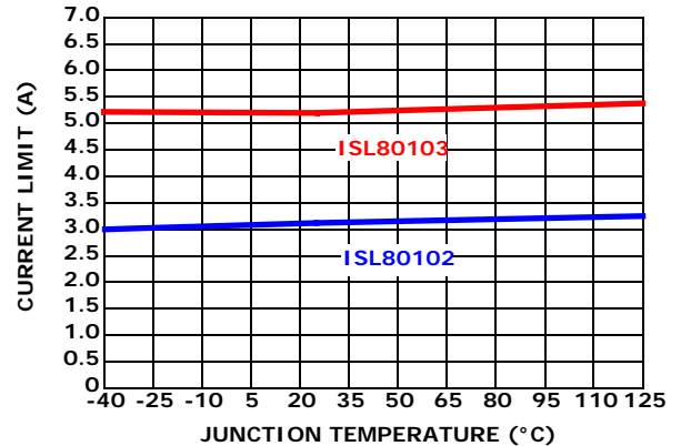
FIGURE 20. CURRENT LIMIT vs TEMPERATURE
