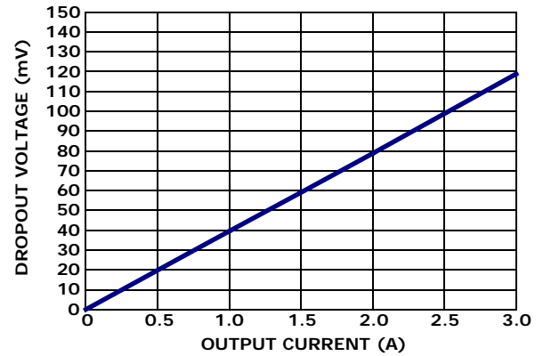
FIGURE 12. DROPOUT VOLTAGE vs OUTPUT CURRENT
