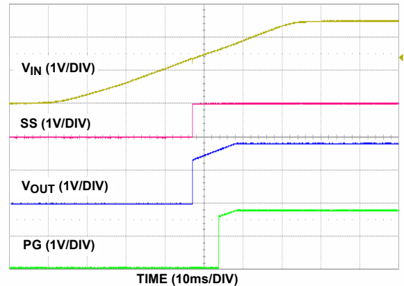
FIGURE 14. POWER-UP ( V_{IN} = 2.2V )
