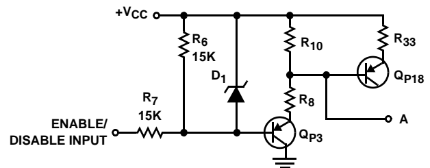
FIGURE 7. SIMPLIFIED SCHEMATIC OF ENABLE/DISABLE FUNCTION
