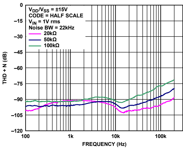
Figure 44. THD + Noise vs. Frequency
